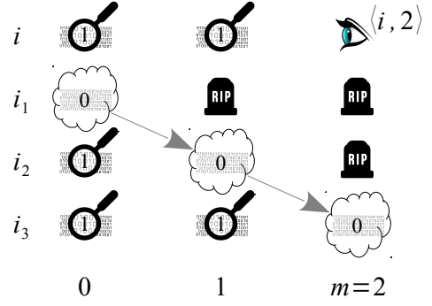
(b) A run i considers at 2 to be possible, in which 0 is held by a correct process at 2.
