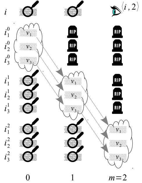
(b) A run i considers at 2 to be possible, in which v_1, v_2, v_3 are held by distinct processes at 2.
