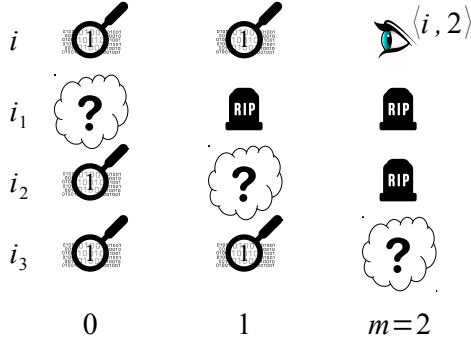
(a) A hidden path w.r.t. \langle i, 2 \rangle .
