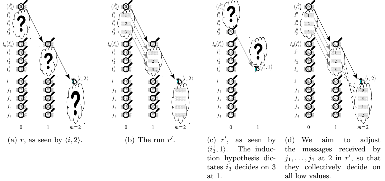
Figure 3: The proof strategy for the induction step of Lemma 1 (for m = 2 , k = 4 ).
