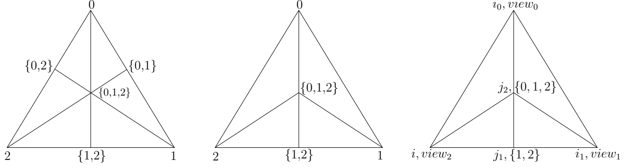
Figure 5: For dimension k = 2 and \sigma = \{0, 1, 2\} , the barycentric subdivision \sigma = \{0, 1, 2\} appears at the left, while the subdivision \text{Div } \sigma appears at the center. In the subdivision at the right, the vertices are mapped to process states. For example, the triangle \{\langle i_0, \text{view}_0 \rangle, \langle i_1, \text{view}_1 \rangle, \langle j_2, \{0, 1, 2\} \rangle\} corresponds to the execution in which i_0 and i_1 do not crash in round m , and hence j_1 receives 0 and 1, which are included in its view. Similarly, the triangle \{\langle i_1, \text{view}_1 \rangle, \langle j_1, \{1, 2\} \rangle, \langle j_2, \{0, 1, 2\} \rangle\} correspond to the execution in which i_1 does not crash in round m , while i_0 crashes and sends a message to j_2 and no message to j_1 . The decisions of the processes induces a Sperner coloring: by assumption, i decides k = 2 , and by induction hypothesis, i_0 and i_1 decided 0 and 1 at time m - 1 ; the rest of the processes have to decide at time m and they can only decide values in their views.
