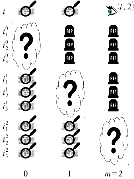
(a) \langle i, 2 \rangle has hidden capacity 3.
