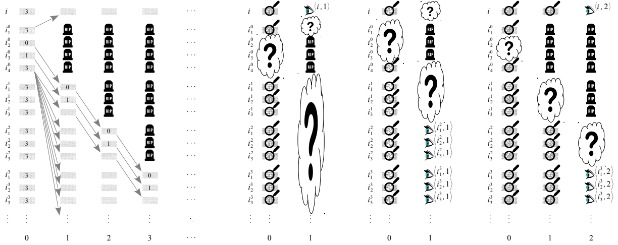
(a) The run r . Messages successfully sent by crashing nodes are marked with an arrow. Starting from time m = 1 , all processes know \exists 3 (i.e., \exists k ), and so only knowledge of additional values is indicated. (b) r , as seen by \langle i, 1 \rangle , which has hidden capacity k = 3 . (c) r , as seen by all other nodes that are nonfaulty at time 1. These nodes also have hidden capacity k = 3 . (These nodes are hidden from one another). (d) r , as seen by all nodes that are nonfaulty at time 2. All such nodes have hidden capacity 2 < k , and furthermore know that their min value (i.e., k ) will persist; thus, they all decide (on k ).
